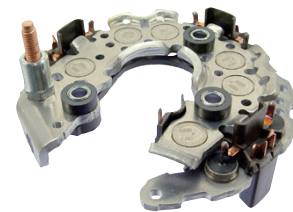
31-82054 Rectifier 117 mm OD M6x1.0 Top Post 100 Amp, 12-50 A Diodes
