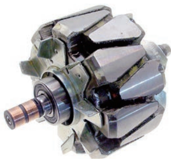
30-82018H37 Rotor 138mm OD Type CW 200 Amp
